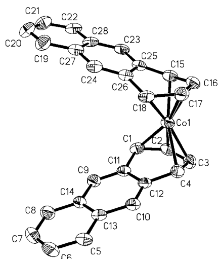
Figure 1. Molecular structure of the anion in 1b . Thermal ellipsoids are set at the 50% probability level, with hydrogen atoms omitted for clarity. Important dimensions [ \text{\AA} and ^\circ ]: Co1–C1 2.125(4), Co1–C2 1.978(4), Co1–C3 2.011(4), Co1–C4 2.132(4), Co1–C15 2.154(4), Co1–C16 2.010(4), Co1–C17 1.974(4), Co1–C18 2.112(4), C1–C2 1.406(5), C2–C3 1.424(5), C3–C4 1.422(5), C15–C16 1.413(5), C16–C17 1.416(5), C17–C18 1.422(5), Co-centroid( \eta^4 ) 1.64; centroid( \eta^4 )–Co-centroid( \eta^4 ) 172.5.
